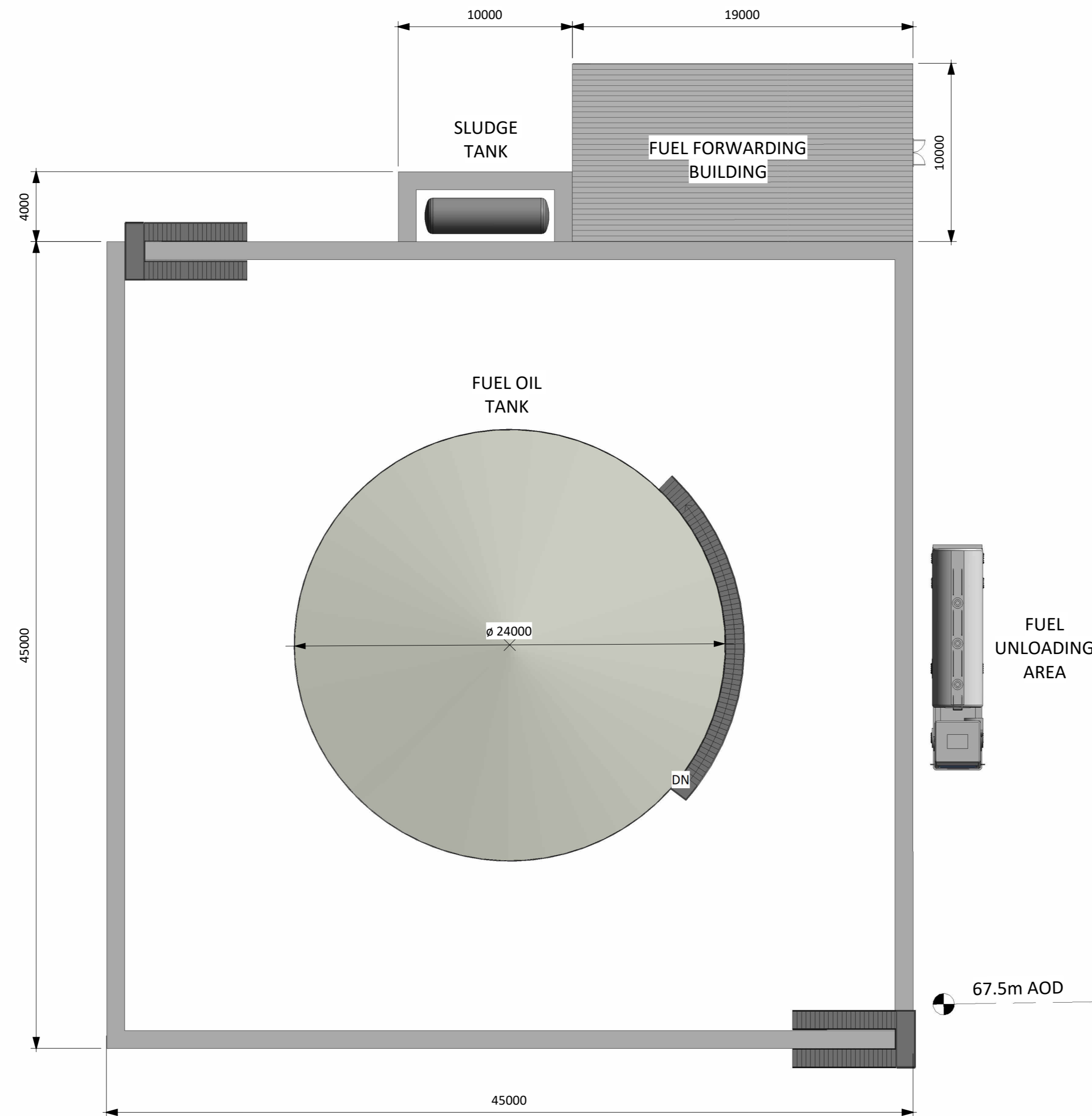
5 Fuel Treatment, Storage and Unloading Plan 1 : 200
