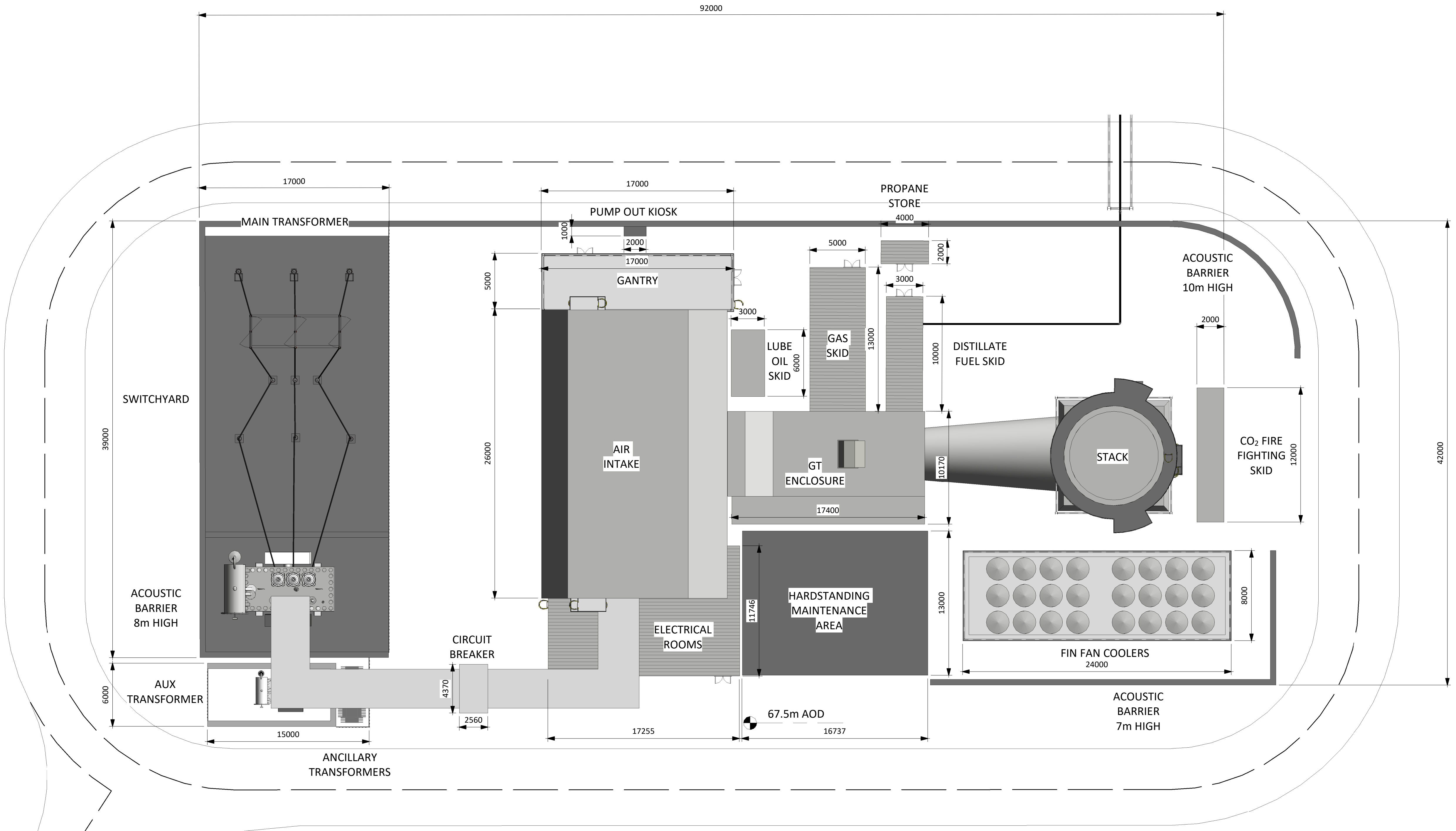
OCGT Key Plan 1:5000
